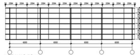
LSC-W10 Pfetten
